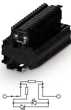
4mm 2 带发光二极管保险管接线端子 Terminal Block With LED Protective Tube
