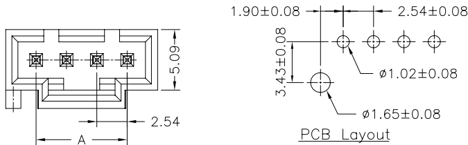
PCB Layout
