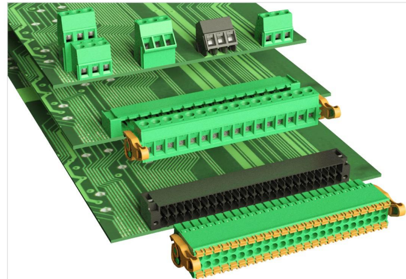
7.62mm间距 Pitch: 7.62mm
