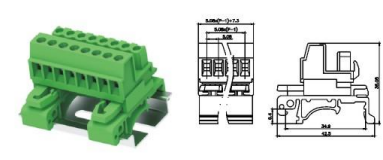
MC-RH5.08HXXC-T-0001
