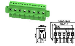
MC-RE7.5VXXC-RK-0001
