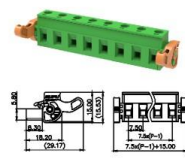
MC-RB7.5HXXC-I-0001
