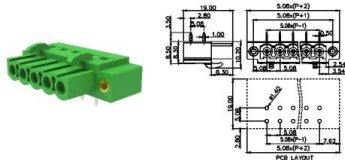
MC-RU5.08SVXX-F-0001
