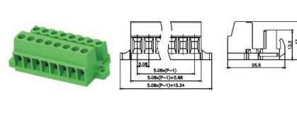
MC-RH5.08HXXC-B-0001
