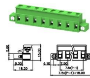
MC-RB7.5HXXC-K-0001
