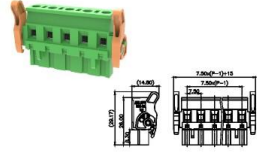
MC-RE7.5VXXC-I-0001
