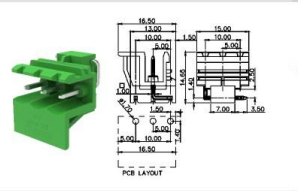
MC-PAR5.0H03-0002
