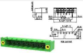
MC-PA5.0HXX-F-0002
