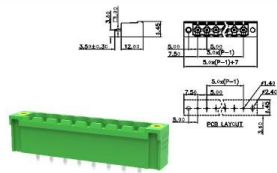
MC-PA5.0HXX-F-0002
