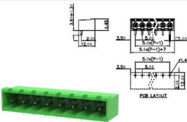
MC-PA5.0HXX-0002
