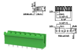
MC-PA5.0HXX-G-0002
