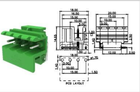
MC-PAR5.0H04-0002
