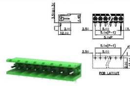
MC-PA5.0HXX-G-0002
