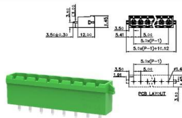
MC-PA5.0HXX-D-0002
