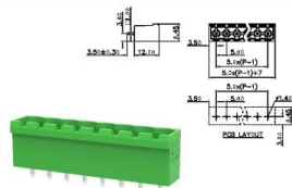
MC-PA5.0HXX-0002
