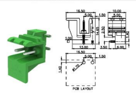
MC-PAR5.0H02-0002
