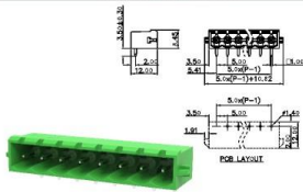
MC-PA5.0HXX-D-0002
